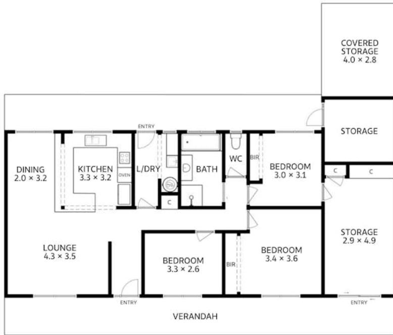
Approx. Floor Area 122 sq m (excluding verandah, spa, covered storage and shed)
